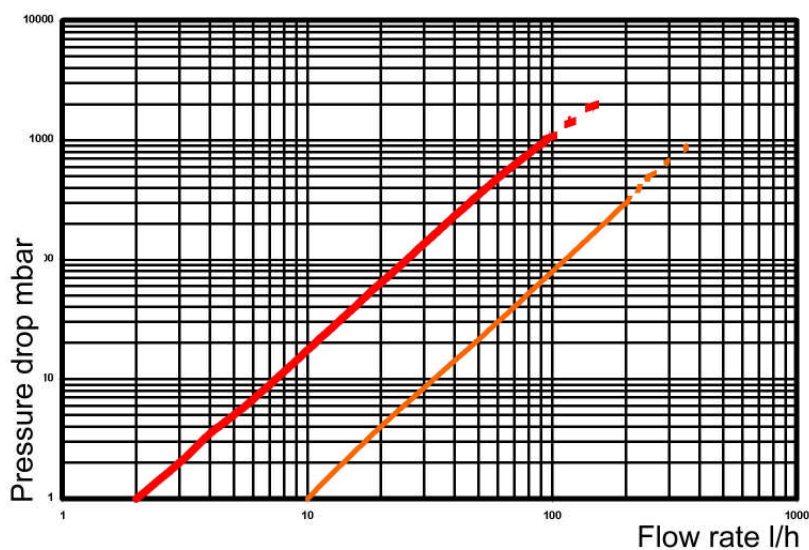
Pressure drop
