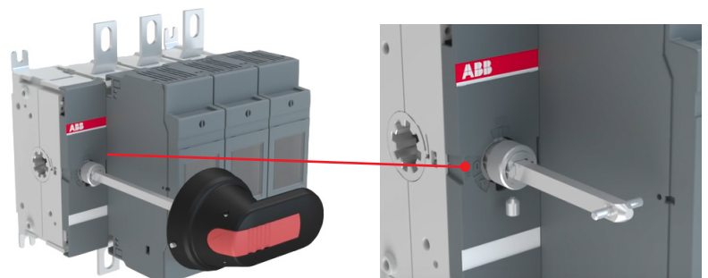
Adjustable shaft
