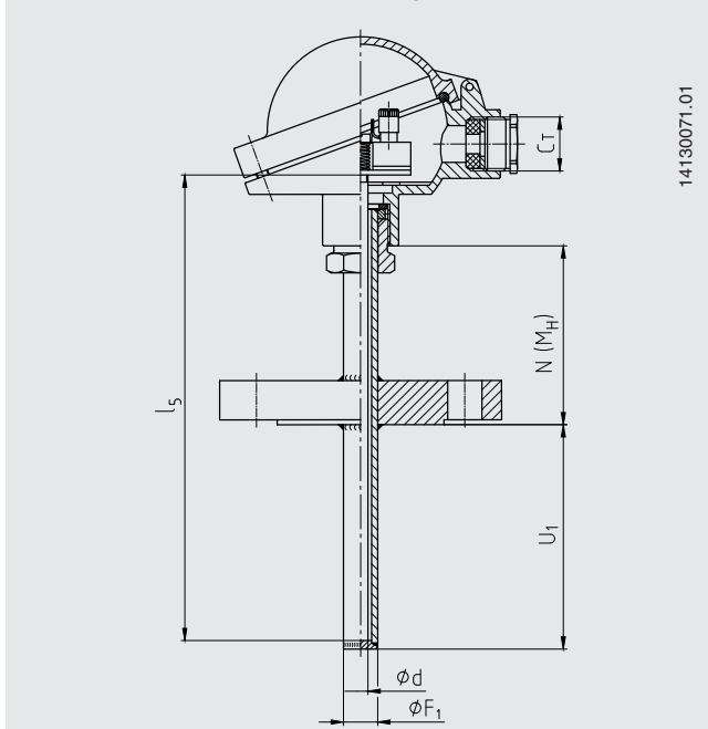
Protection tube model TW40, straight, form 2F DIN 43772
