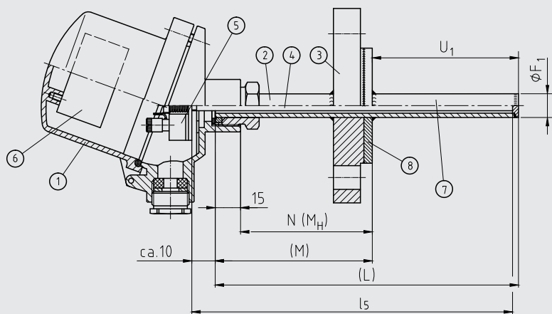
Version: Flange from standard material, protection tube and flange disc from special materials
