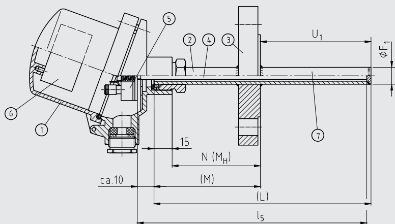
Version: Flanged protection tube from standard material
