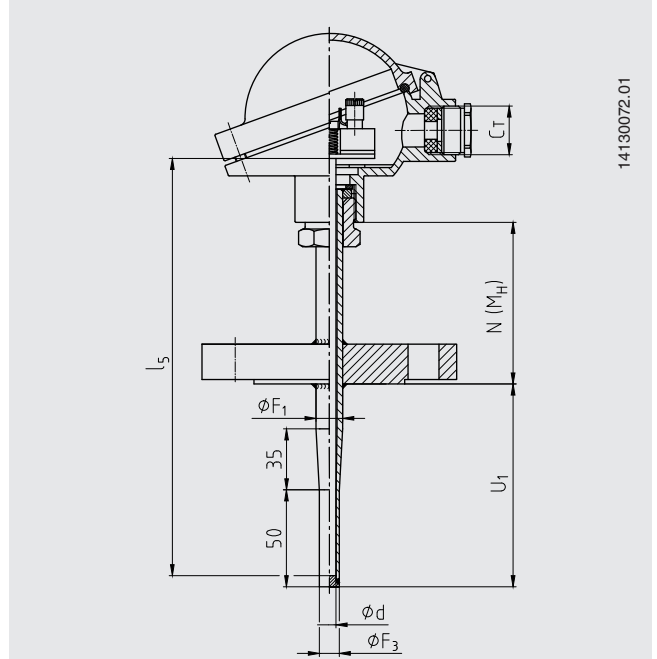
Protection tube model TW40, tapered, form 3F DIN 43772
