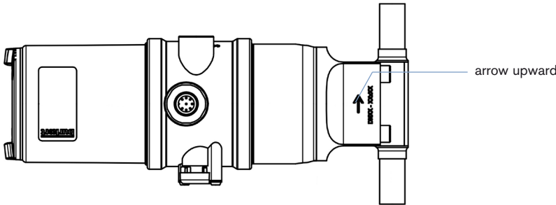
Fig. 1: Installation position for self-draining
