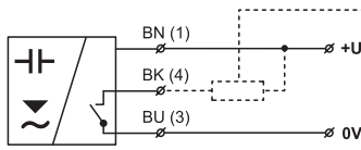
Fig. 7: NPN type sensors connection (version "N")
