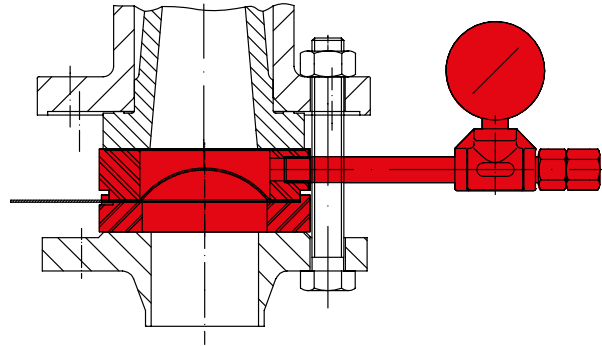
Rupture disc
