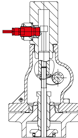
Proximity switch
