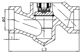
Fig. 149....111....3 / ....112....3 with socket weld ends
