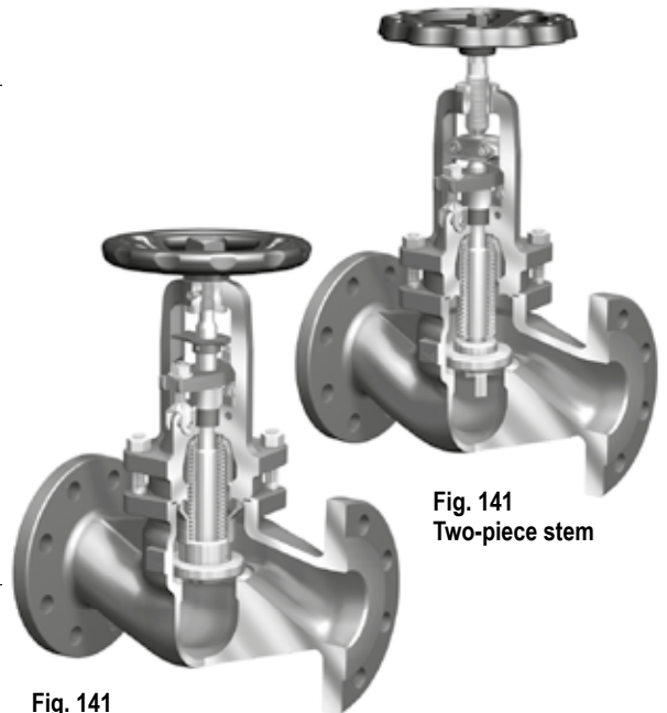
Fig. 141 One-piece stem
