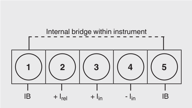
5-pin terminal block
